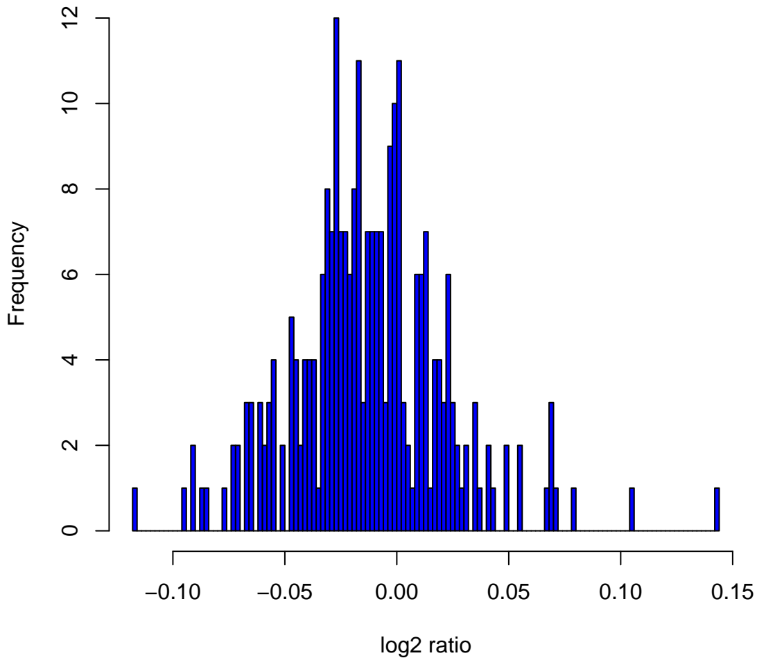
Histogram of \log_2 ratios in 270 HapMap samples at clone Chr2tp-4H7
