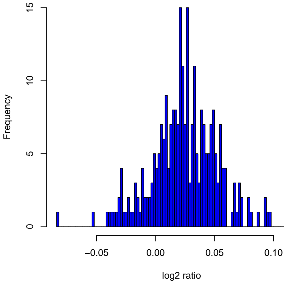
Histogram of log 2 ratios in 270 HapMap samples at clone Chr2tp-4H8
