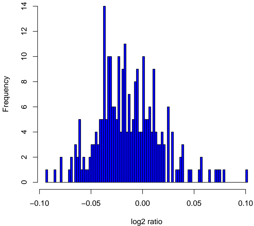
Histogram of log 2 ratios in 270 HapMap samples at clone Chr2tp-5D5
