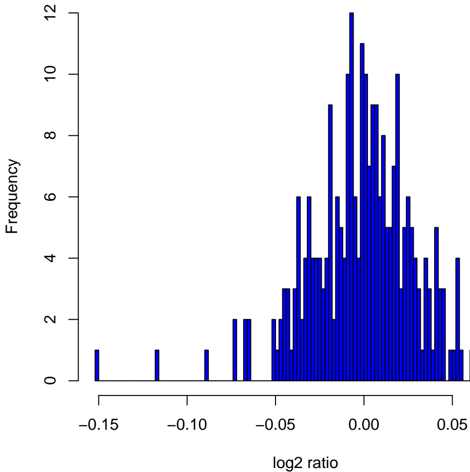
Histogram of log2ratios in 270 HapMap samples at clone Chr2tp-5E5
