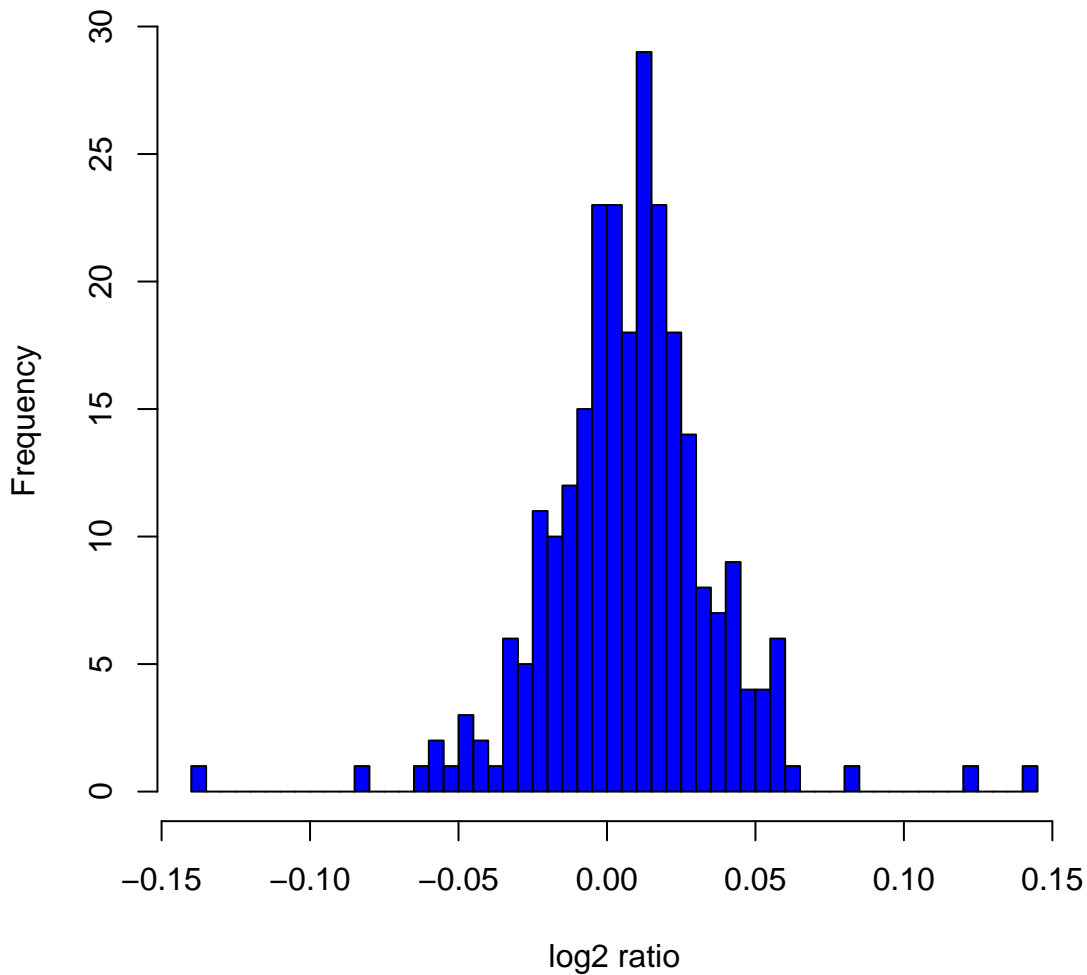
Histogram of log 2 ratios in 270 HapMap samples at clone Chr2tp-5E8
