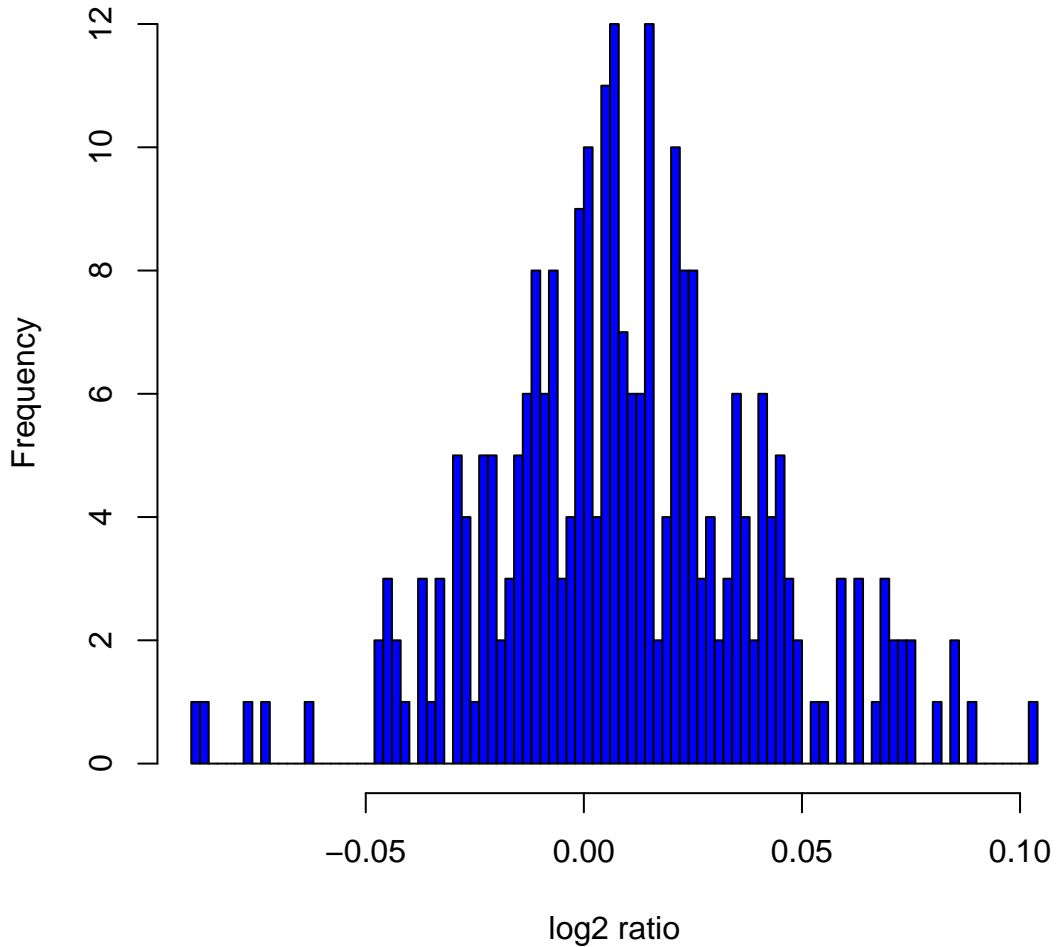
Histogram of log2ratios in 270 HapMap samples at clone Chr2tp-5F2
