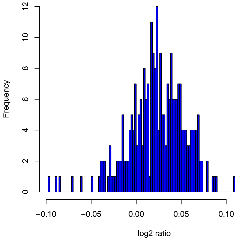
Histogram of \log_2 ratios in 270 HapMap samples at clone Chr2tp-5G6
