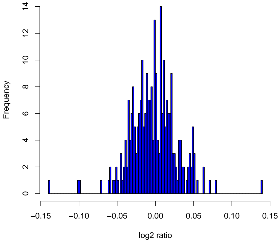
Histogram of log 2 ratios in 270 HapMap samples at clone Chr2tp-5G8
