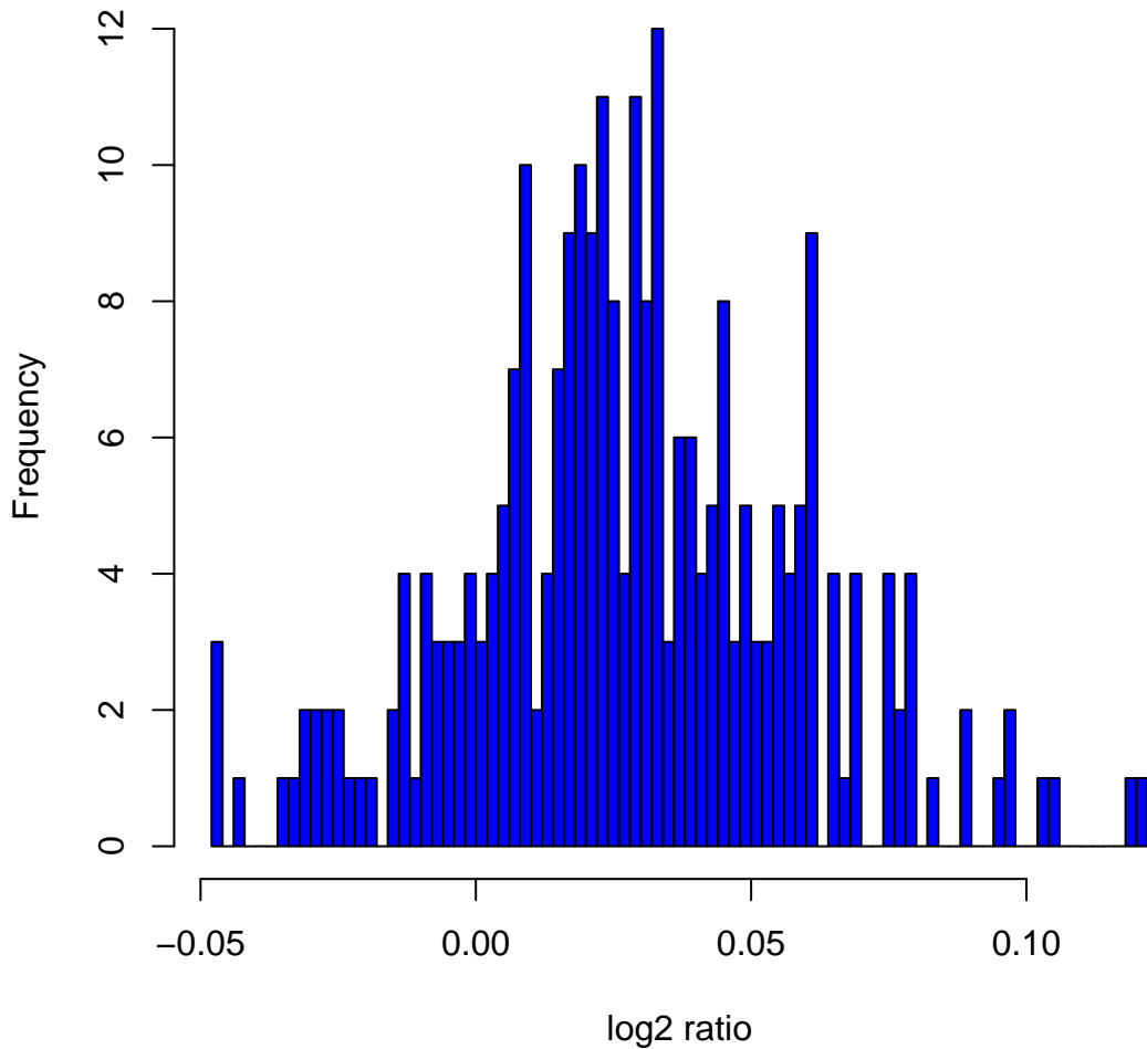
Histogram of log 2 ratios in 270 HapMap samples at clone Chr2tp-5H9
