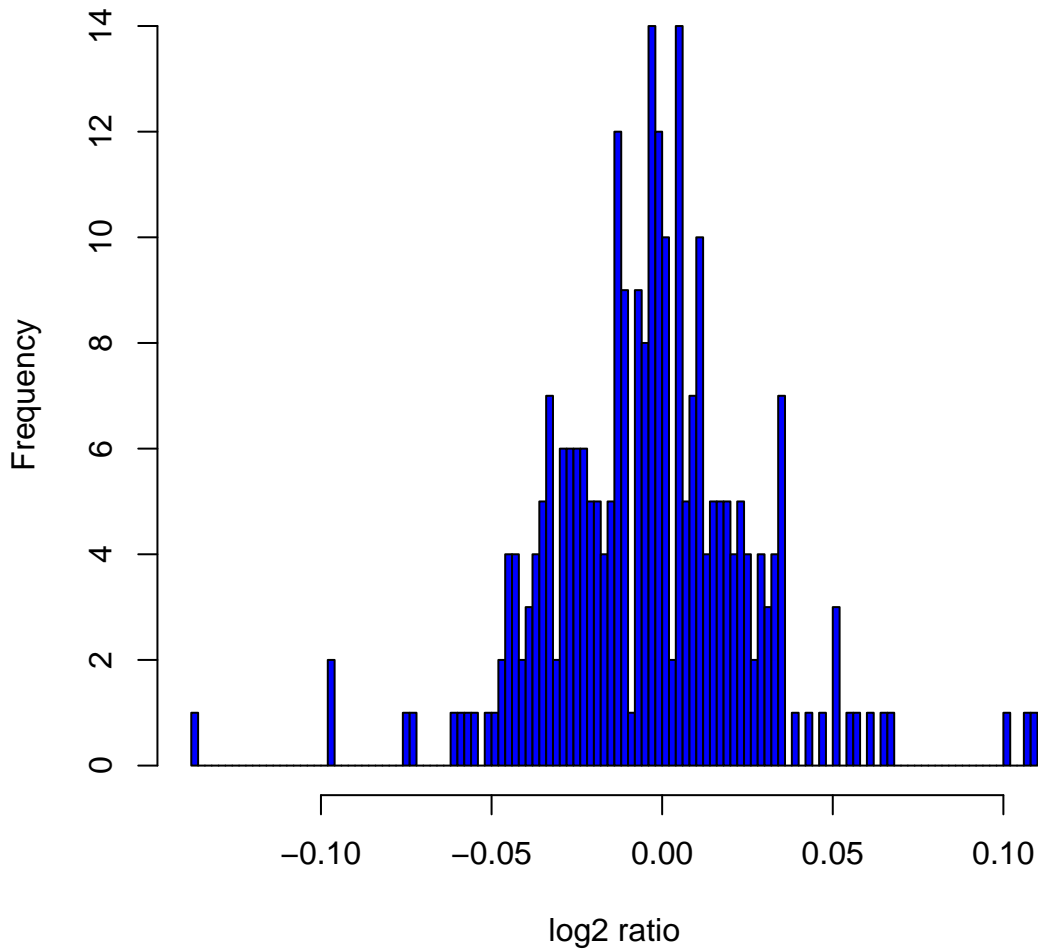
Histogram of \log_2 ratios in 270 HapMap samples at clone Chr2tp-6A1
