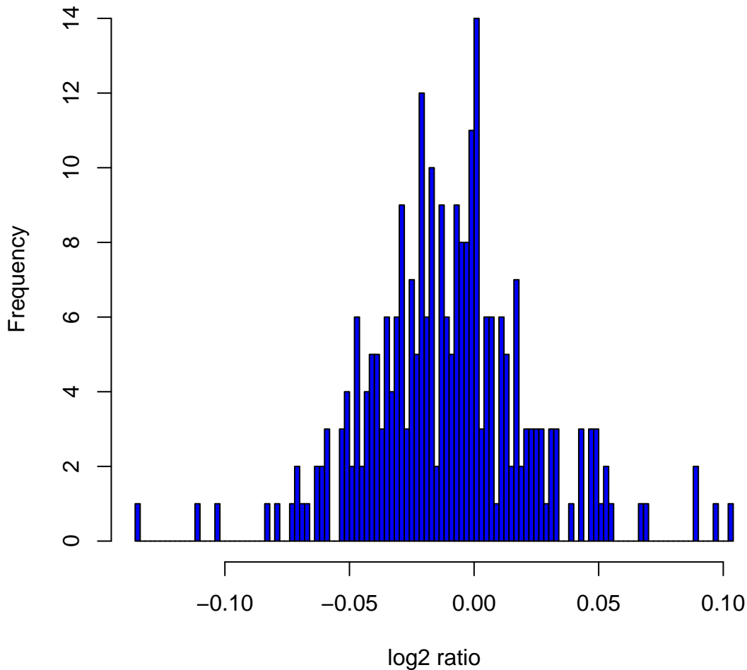
Histogram of log 2 ratios in 270 HapMap samples at clone Chr2tp-6E4
