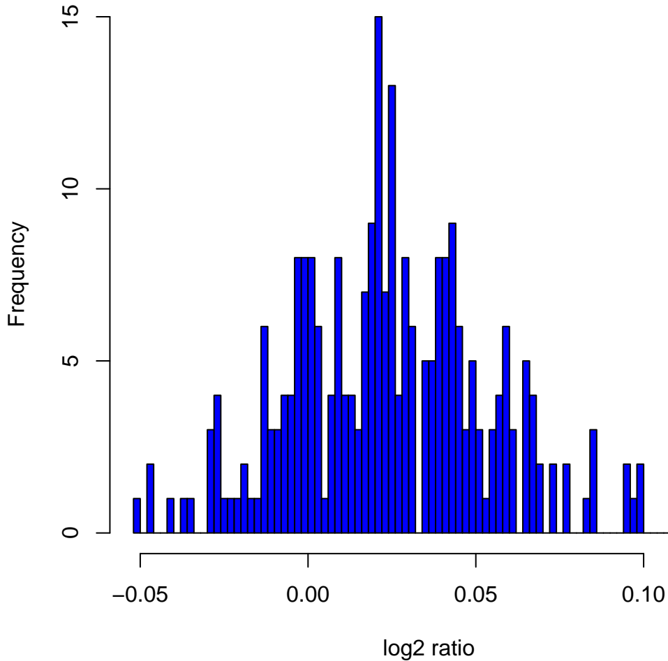
Histogram of log2ratios in 270 HapMap samples at clone Chr2tp-6F2
