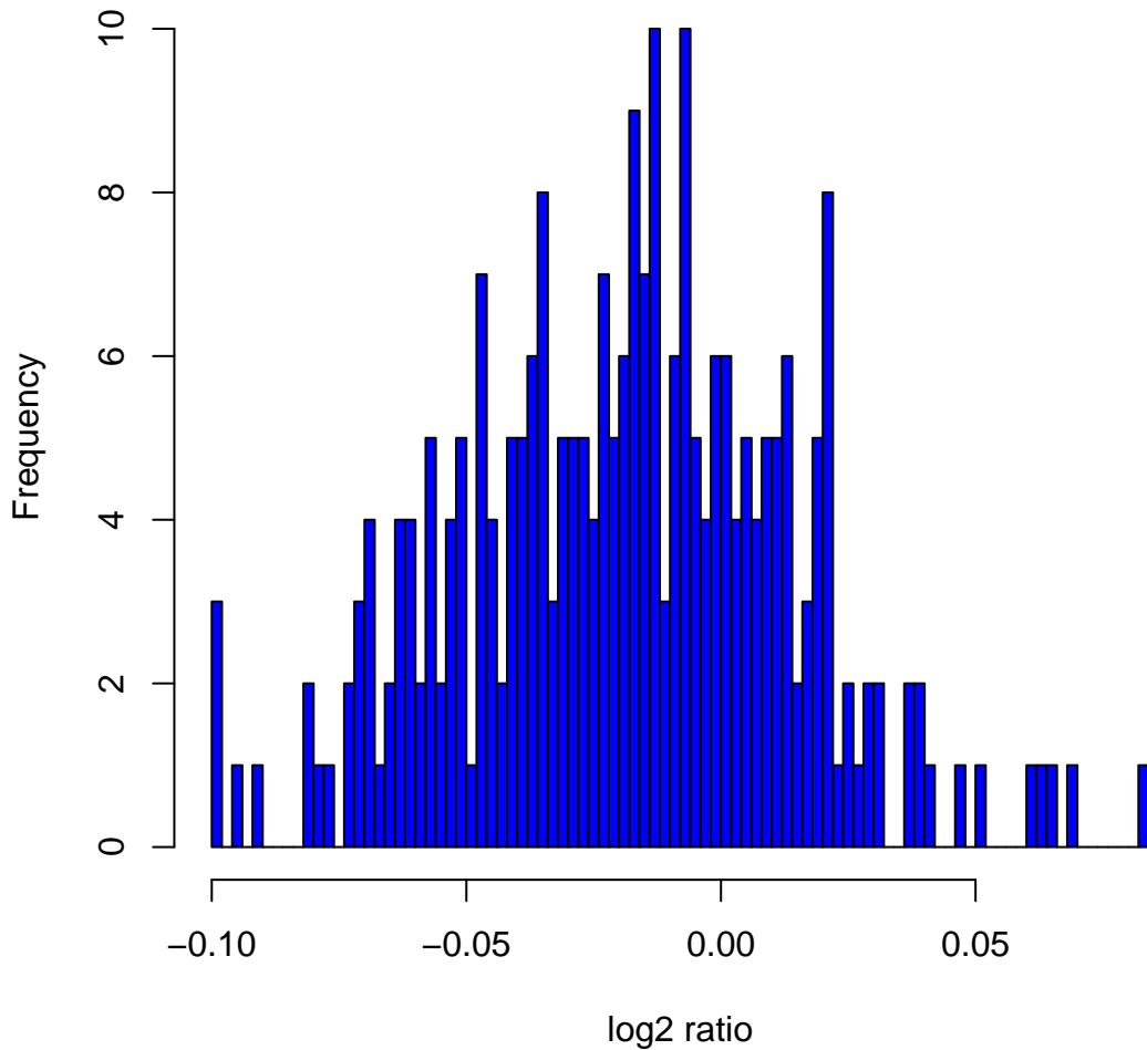
Histogram of log 2 ratios in 270 HapMap samples at clone Chr2tp-6G11
