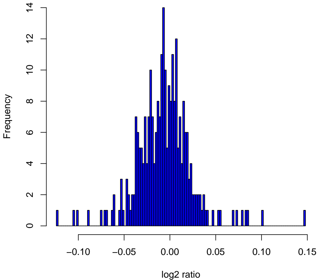
Histogram of \log_2 ratios in 270 HapMap samples at clone Chr2tp-6G4
