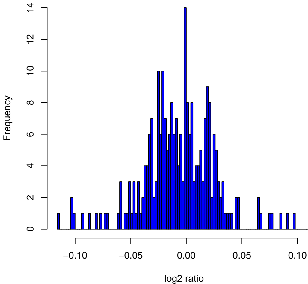
Histogram of log 2 ratios in 270 HapMap samples at clone Chr2tp-6H6
