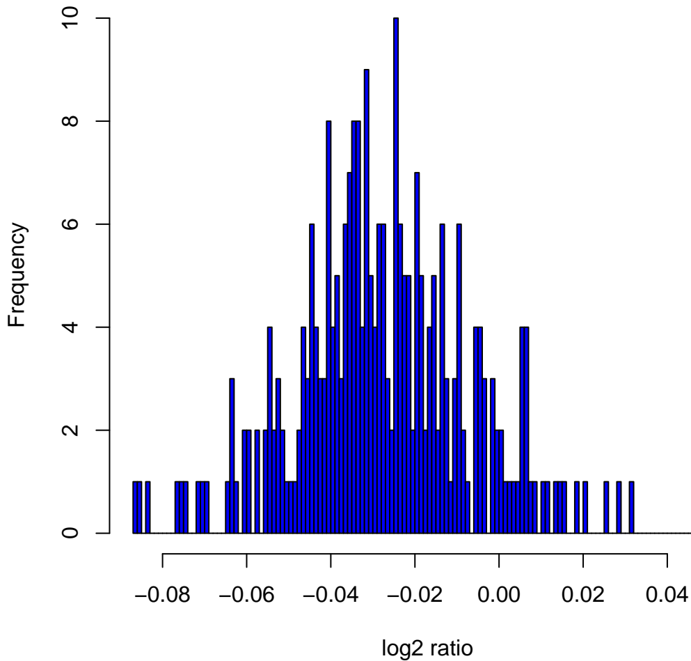
Histogram of \log_2 ratios in 270 HapMap samples at clone Chr2tp-7C4
