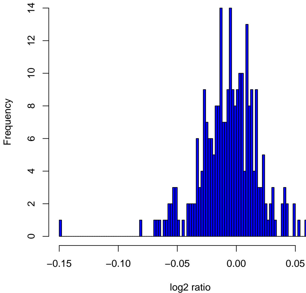
Histogram of log 2 ratios in 270 HapMap samples at clone Chr2tp-7C8
