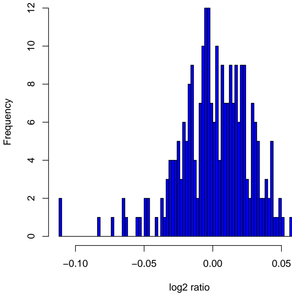
Histogram of \log_2 ratios in 270 HapMap samples at clone Chr2tp-7D7
