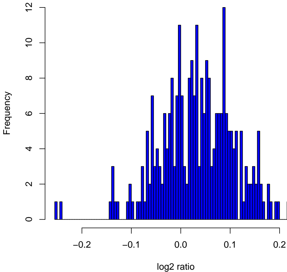
Histogram of log 2 ratios in 270 HapMap samples at clone Chr2tp-7E6
