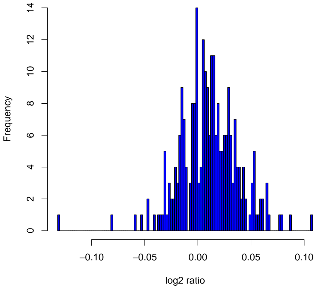
Histogram of log 2 ratios in 270 HapMap samples at clone Chr2tp-7H3
