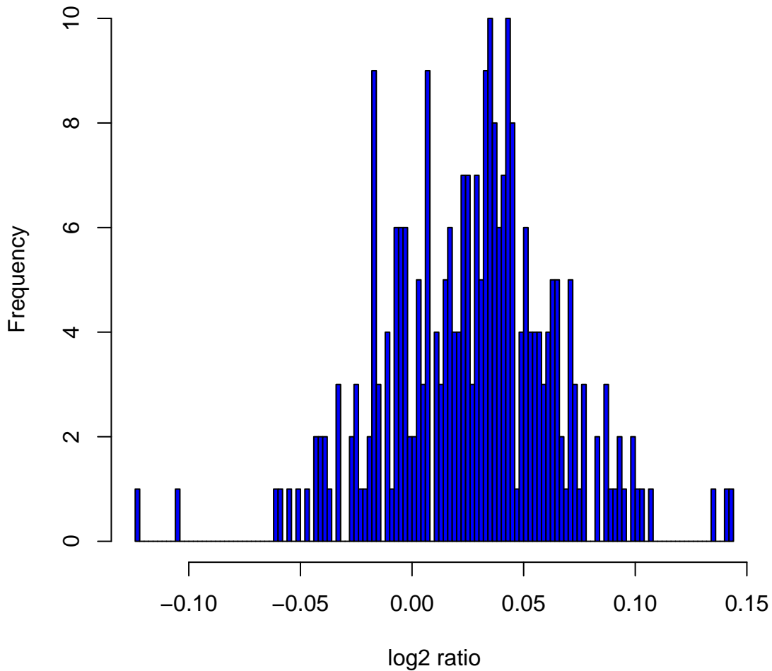
Histogram of log 2 ratios in 270 HapMap samples at clone Chr2tp-8A3
