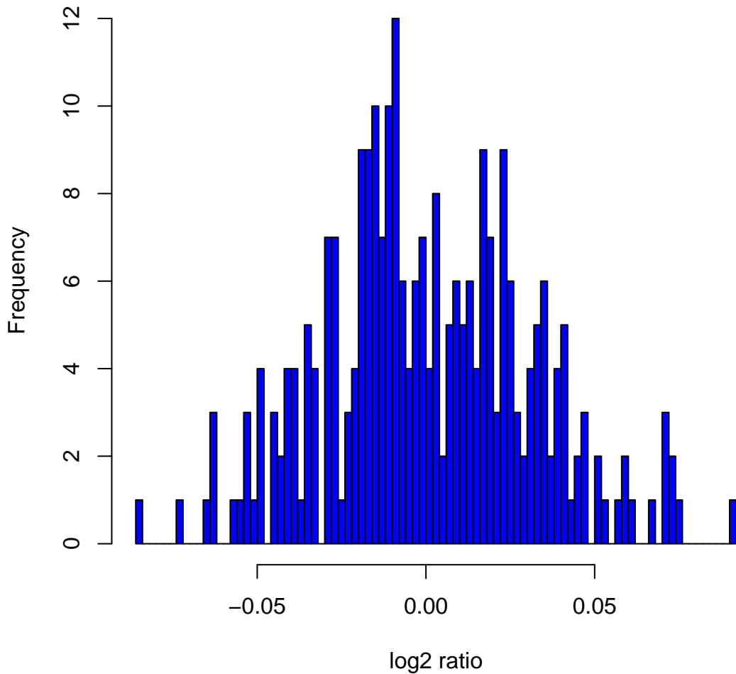
Histogram of log 2 ratios in 270 HapMap samples at clone Chr2tp-8A9
