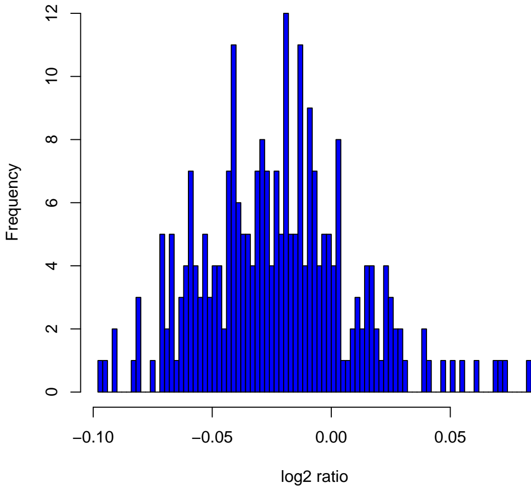
Histogram of log 2 ratios in 270 HapMap samples at clone Chr2tp-8B2
