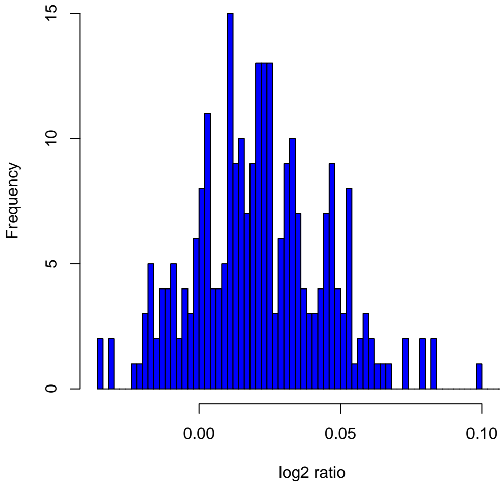
Histogram of log 2 ratios in 270 HapMap samples at clone Chr2tp-8D6
