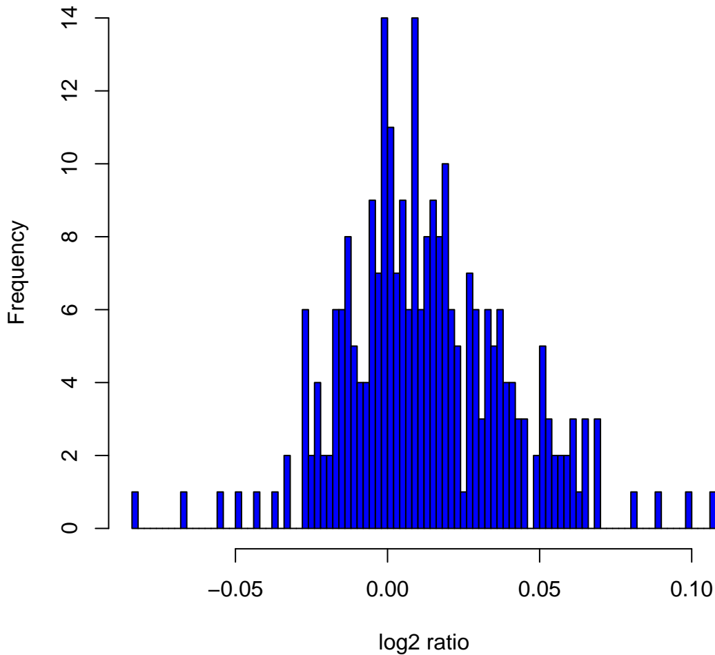
Histogram of log 2 ratios in 270 HapMap samples at clone Chr2tp-8G1
