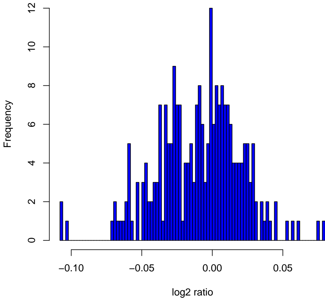
Histogram of \log_2 ratios in 270 HapMap samples at clone Chr2tp-8H7
