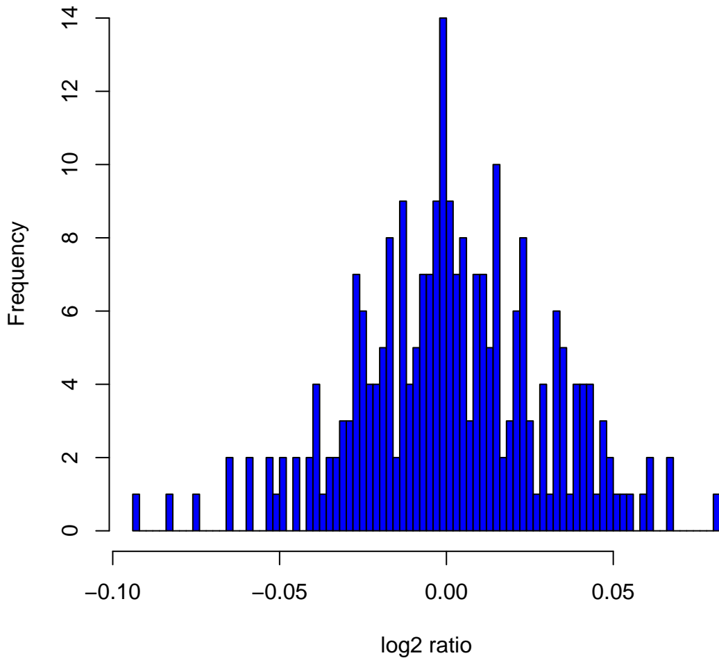
Histogram of log 2 ratios in 270 HapMap samples at clone Chr2tp-9B1
