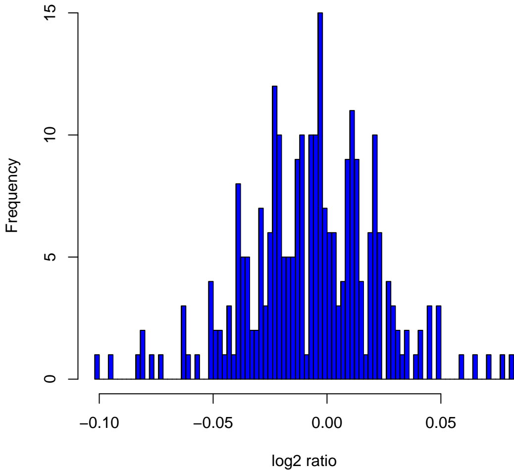
Histogram of \log_2 ratios in 270 HapMap samples at clone Chr2tp-9B4
