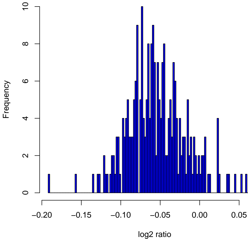
Histogram of \log_2 ratios in 270 HapMap samples at clone Chr2tp-9D7
