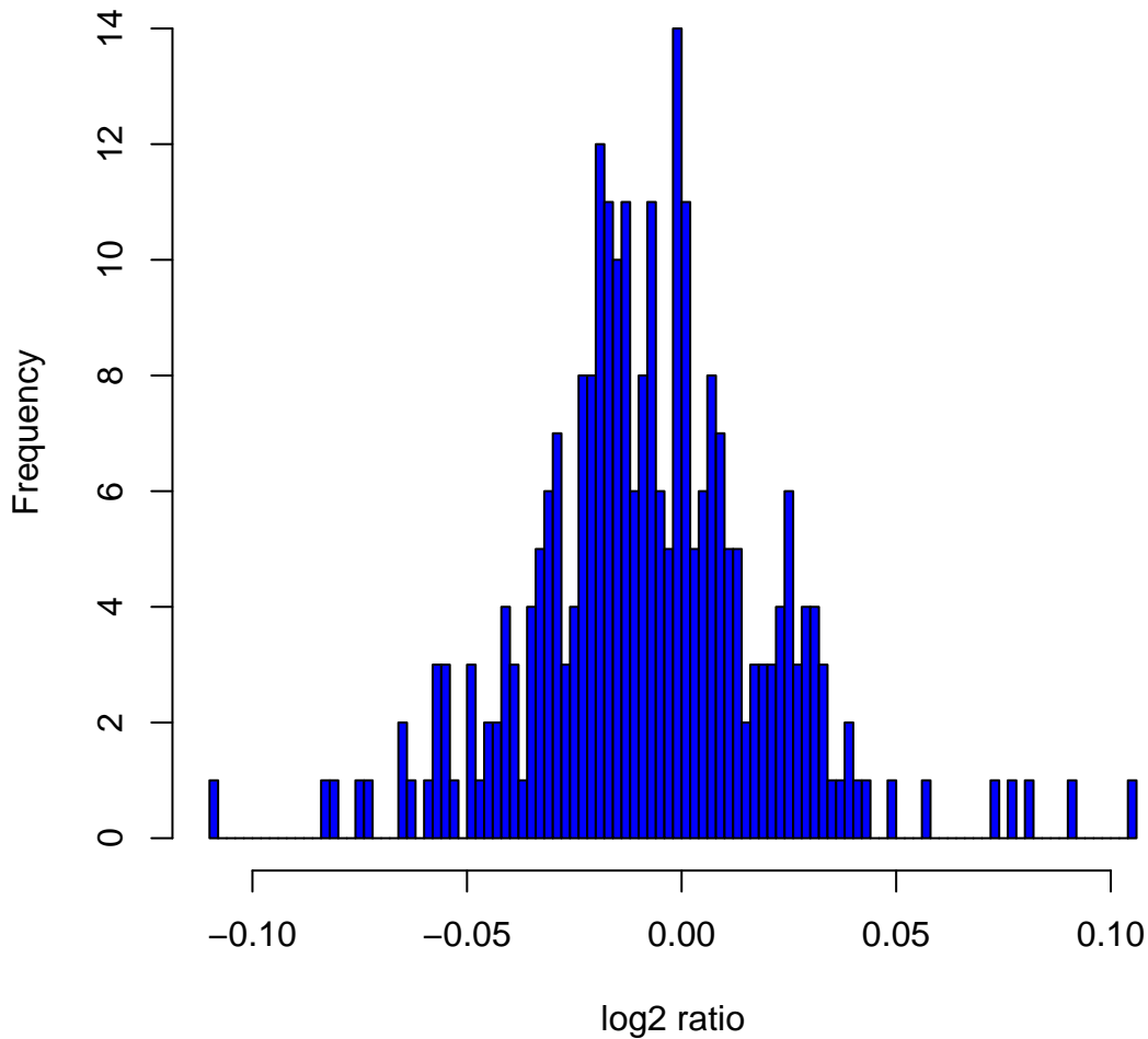
Histogram of log 2 ratios in 270 HapMap samples at clone Chr2tp-9E10
