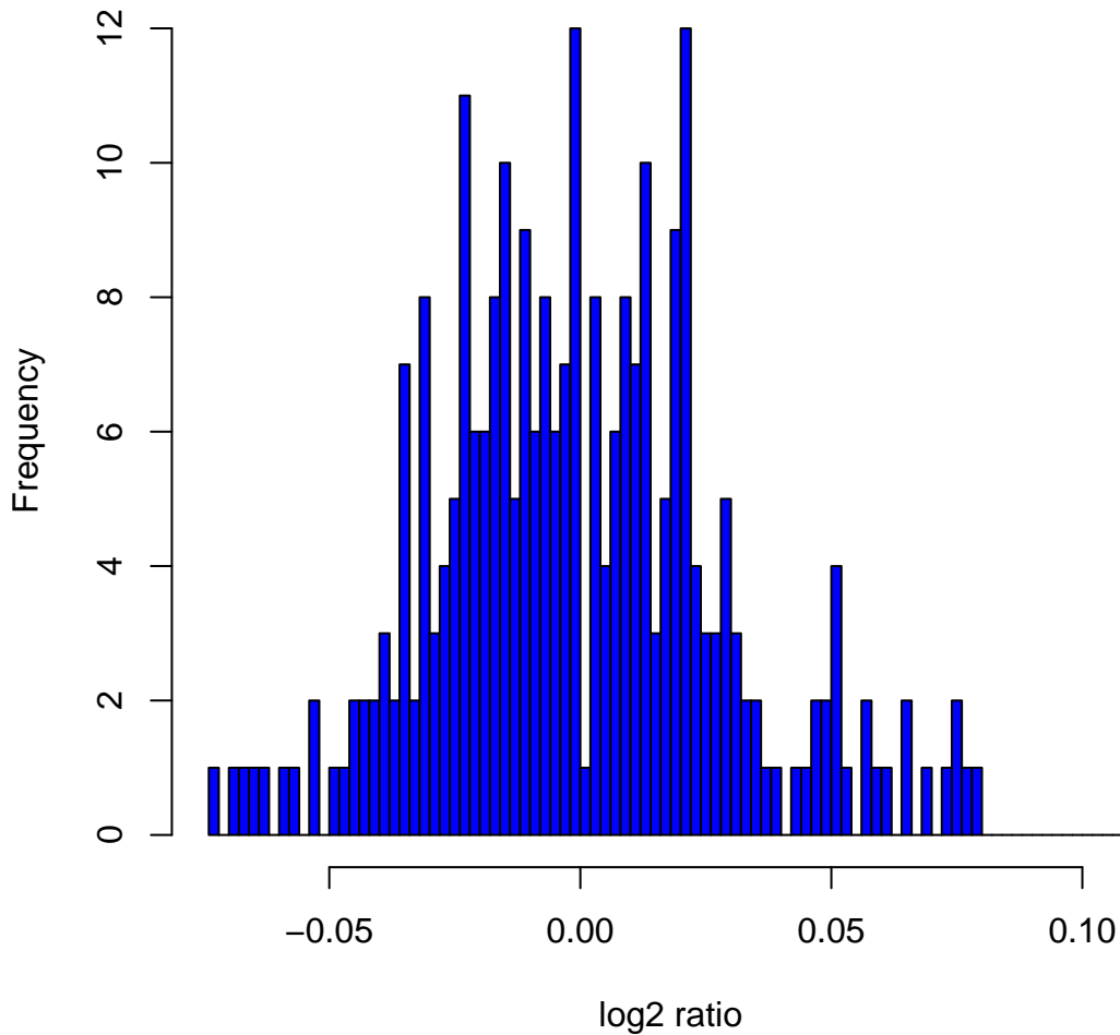
Histogram of log 2 ratios in 270 HapMap samples at clone Chr2tp-9E2
