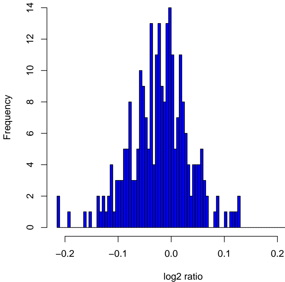
Histogram of log 2 ratios in 270 HapMap samples at clone Chr2tp-9F5
