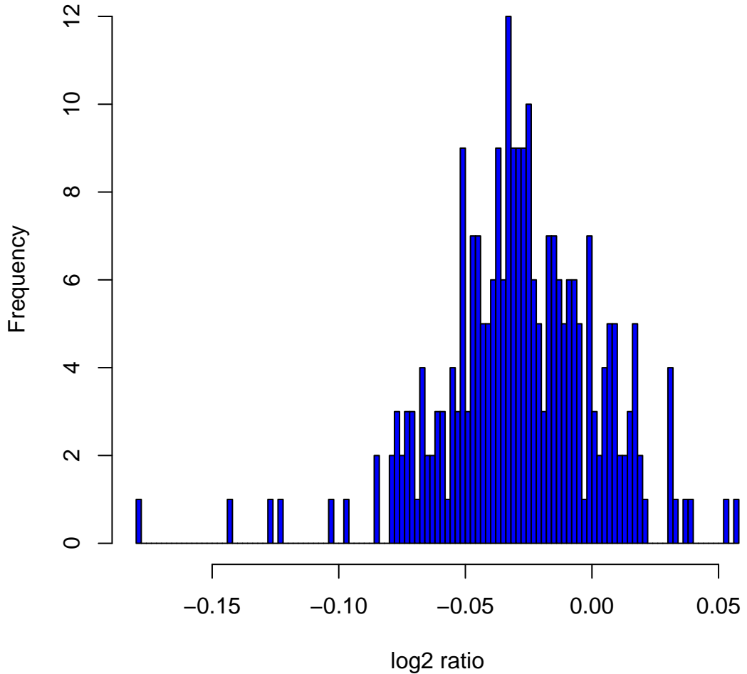
Histogram of log 2 ratios in 270 HapMap samples at clone Chr2tp-9F8
