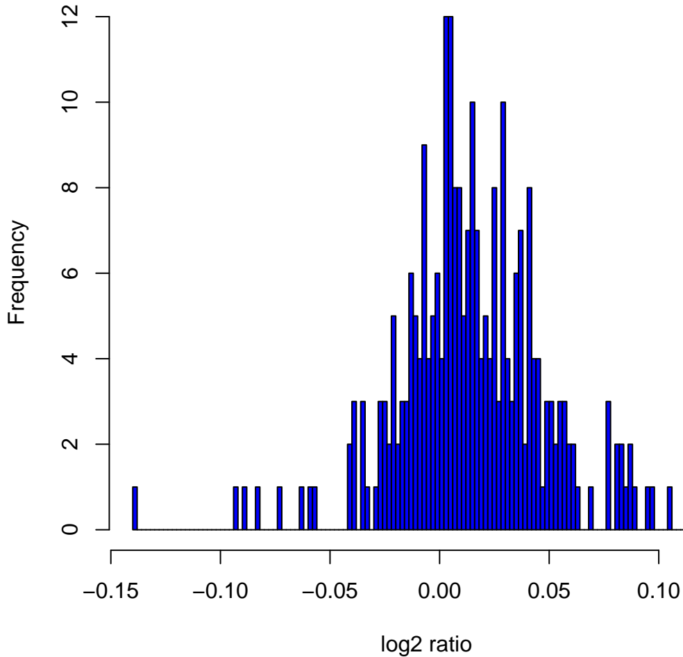
Histogram of log2ratios in 270 HapMap samples at clone Chr2tp-9F9
