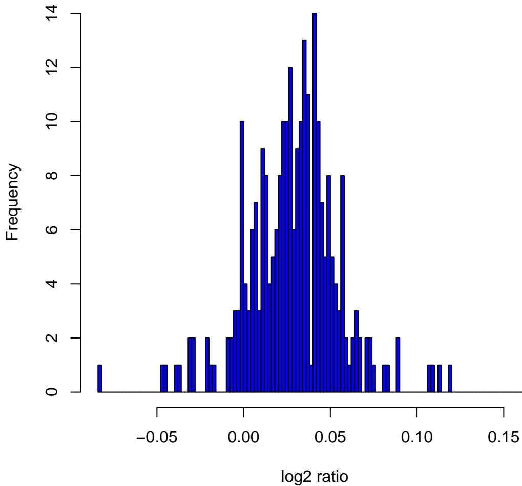
Histogram of log2ratios in 270 HapMap samples at clone Chr2tp-9G10
