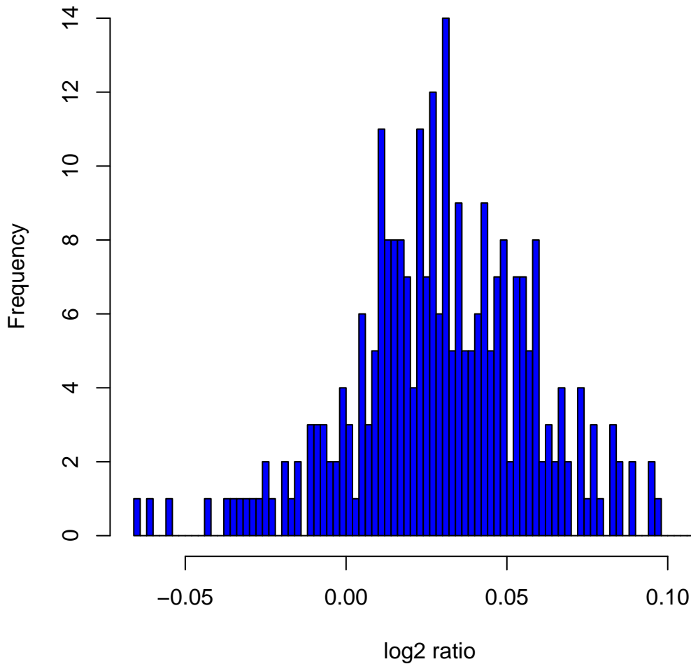
Histogram of log2ratios in 270 HapMap samples at clone Chr22tp-10A4
