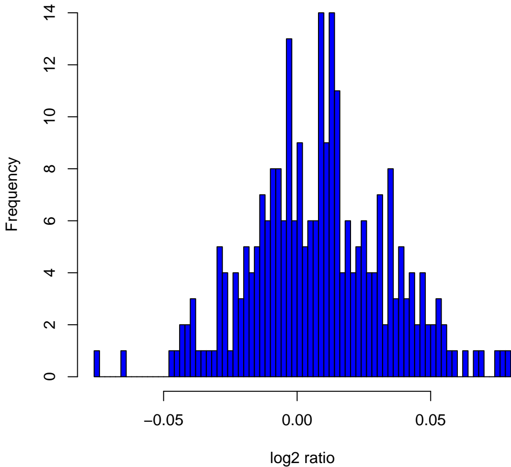
Histogram of log2ratios in 270 HapMap samples at clone Chr22tp-10D4
