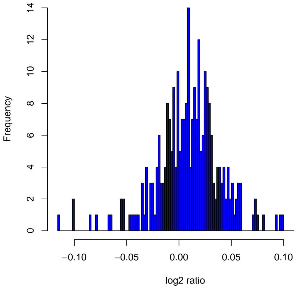
Histogram of log2ratios in 270 HapMap samples at clone Chr22tp-10D6
