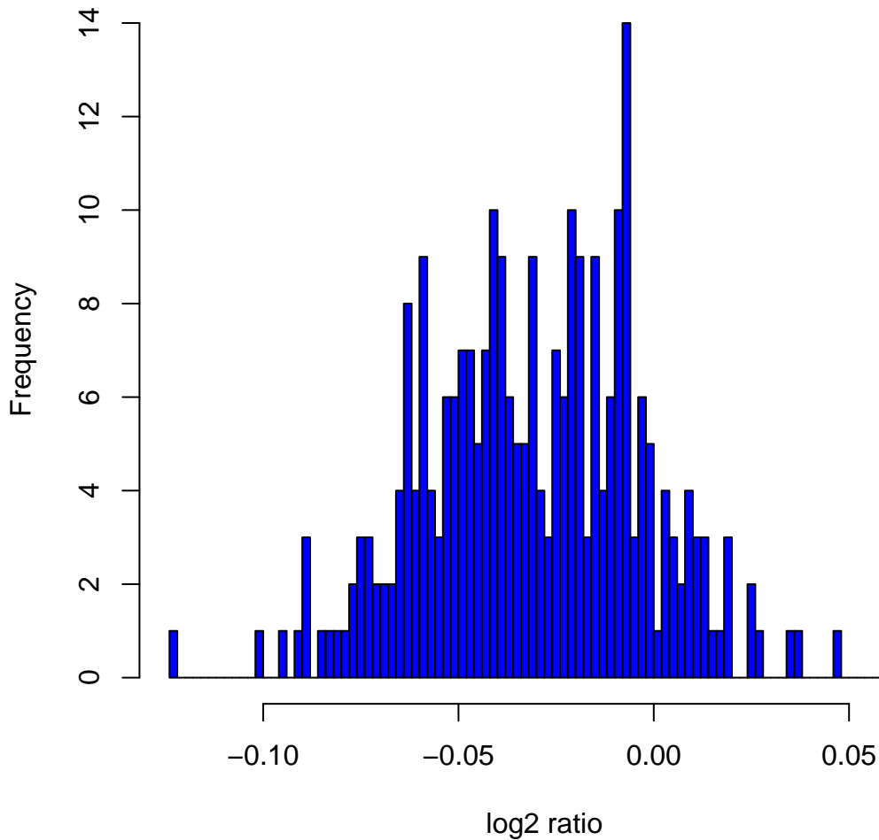
Histogram of log2ratios in 270 HapMap samples at clone Chr22tp-10E6
