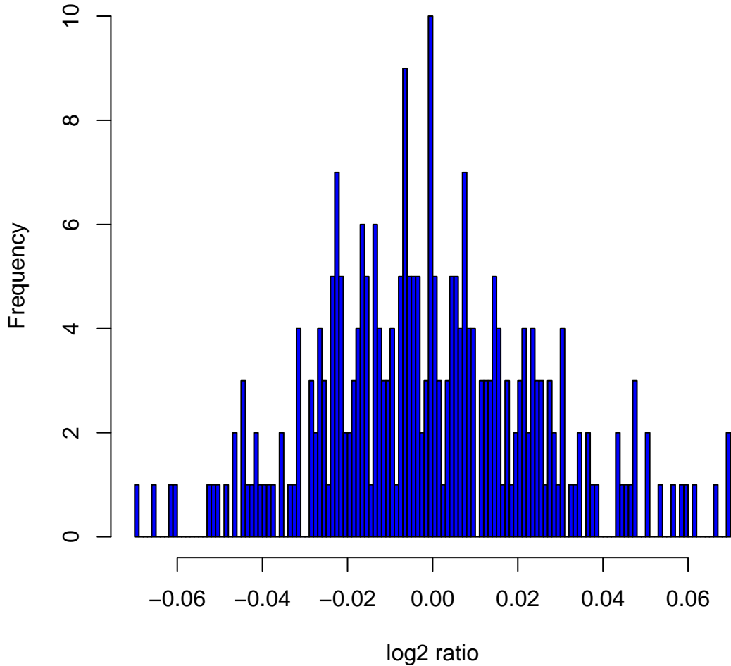
Histogram of log2ratios in 270 HapMap samples at clone Chr22tp-10E9
