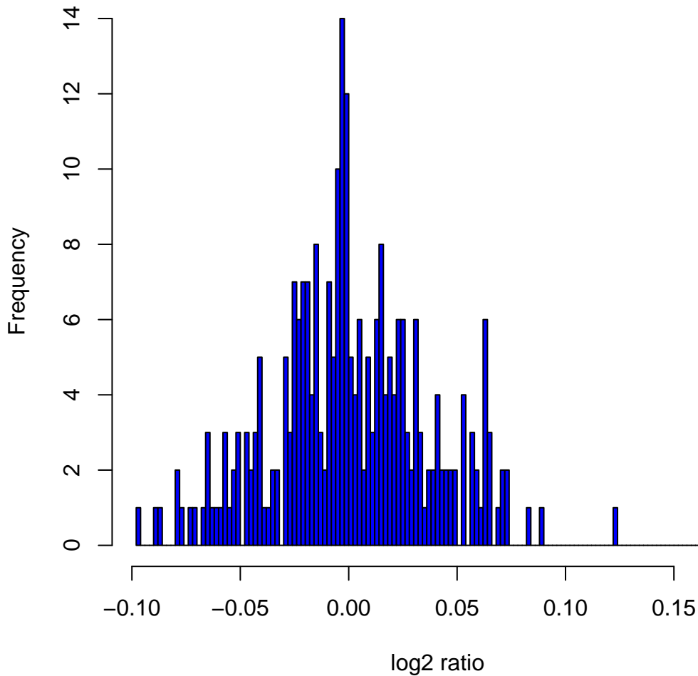
Histogram of log2ratios in 270 HapMap samples at clone Chr22tp-11A6
