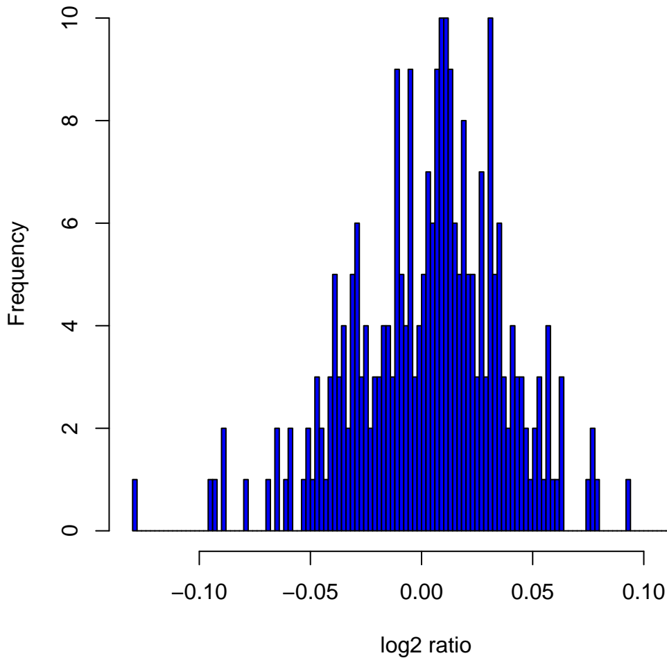
Histogram of log 2 ratios in 270 HapMap samples at clone Chr22tp-2A6
