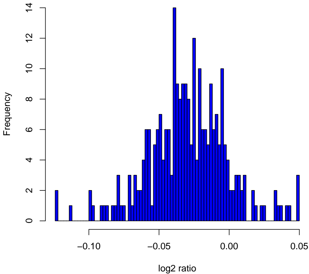
Histogram of log2ratios in 270 HapMap samples at clone Chr22tp-2C9
