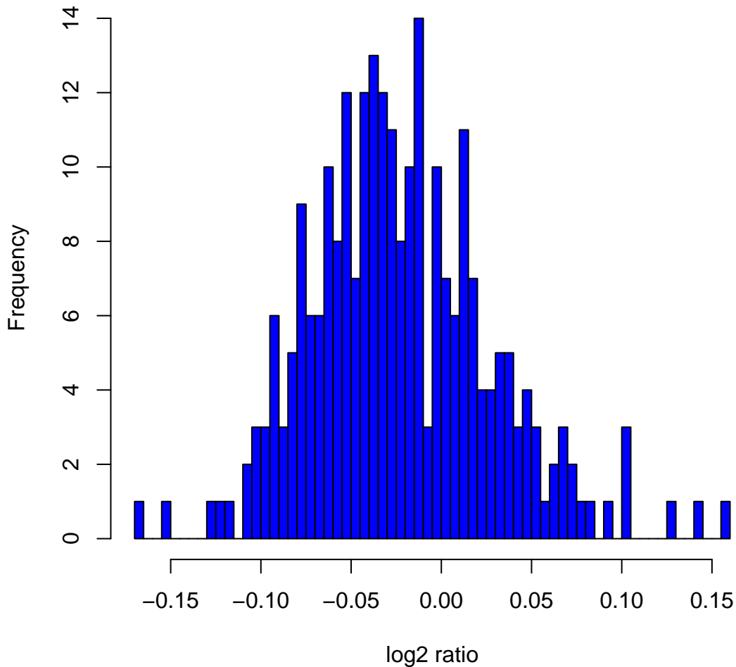
Histogram of log2ratios in 270 HapMap samples at clone Chr22tp-2F11
