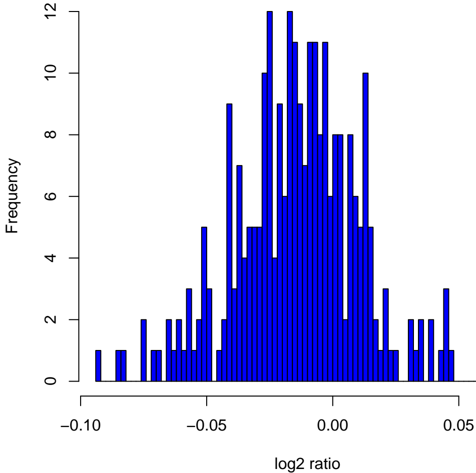
Histogram of log 2 ratios in 270 HapMap samples at clone Chr22tp-2G3
