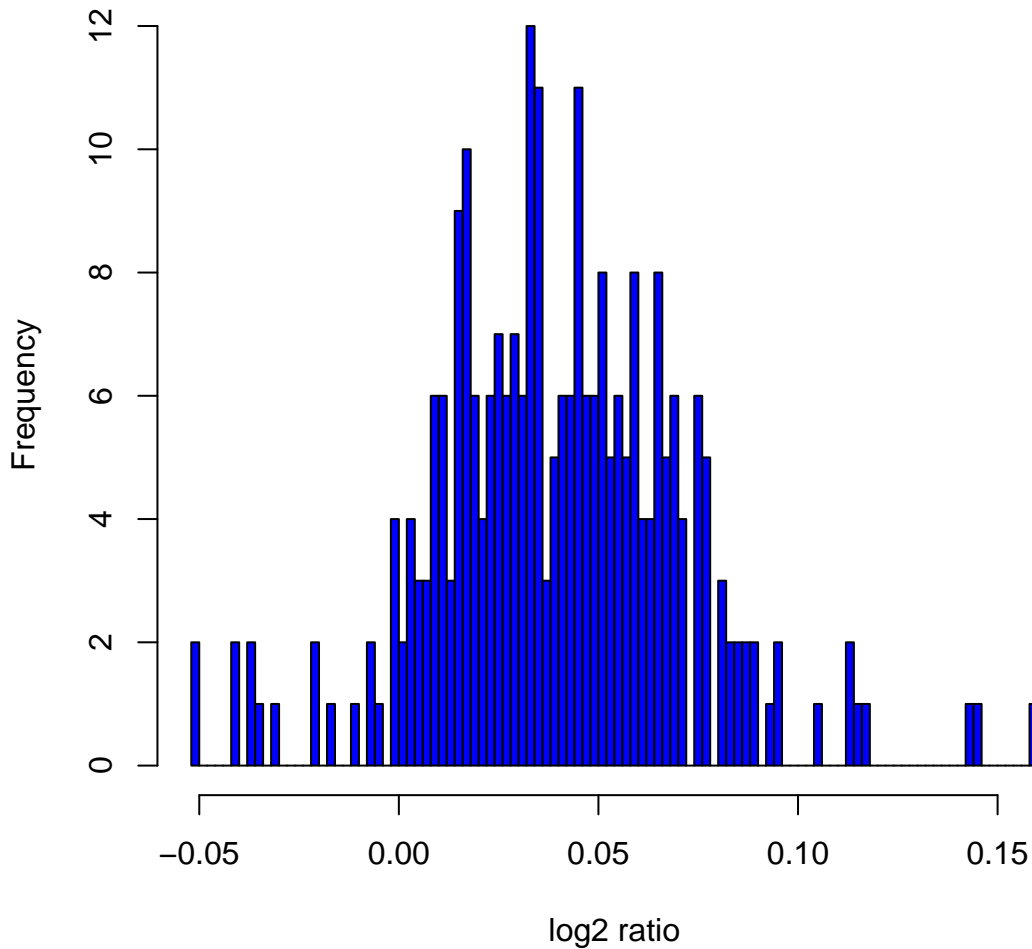
Histogram of log 2 ratios in 270 HapMap samples at clone Chr22tp-3E6
