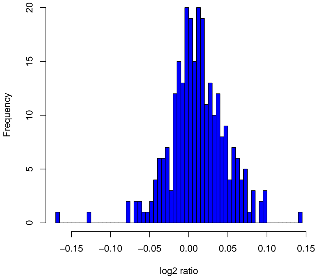
Histogram of log2ratios in 270 HapMap samples at clone Chr22tp-4A12
