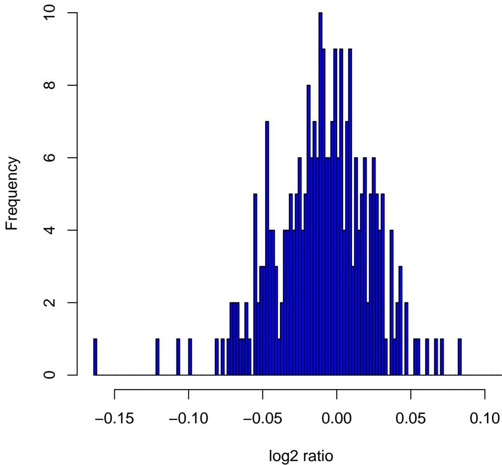
Histogram of log 2 ratios in 270 HapMap samples at clone Chr22tp-5A1
