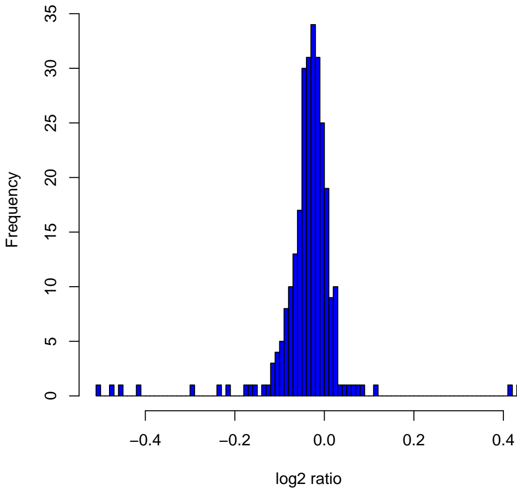
Histogram of log 2 ratios in 270 HapMap samples at clone Chr22tp-6B8
