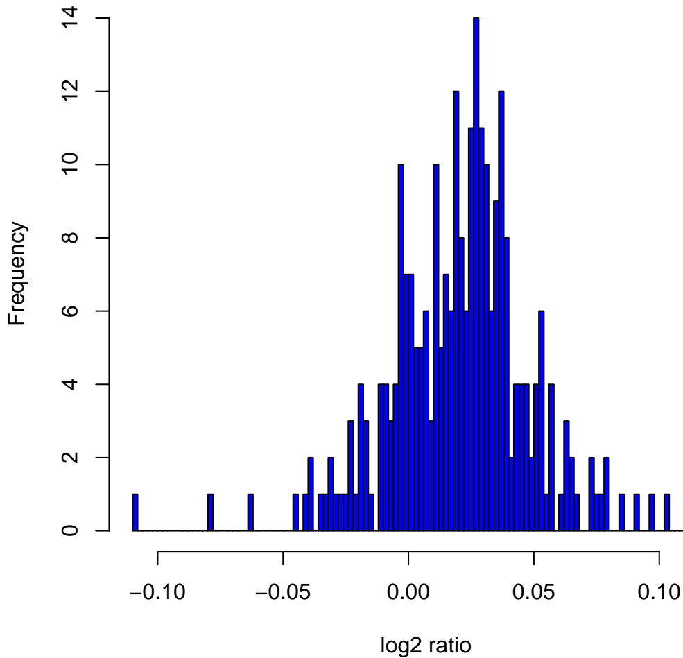
Histogram of log 2 ratios in 270 HapMap samples at clone Chr22tp-8A9
